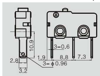
Quick-connect Terminals (#110)
