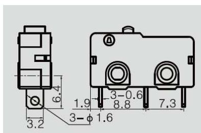
Solder Terminals
