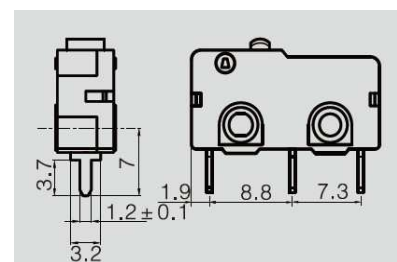
PCB Terminals
