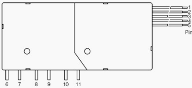
单线圈 Single coil
